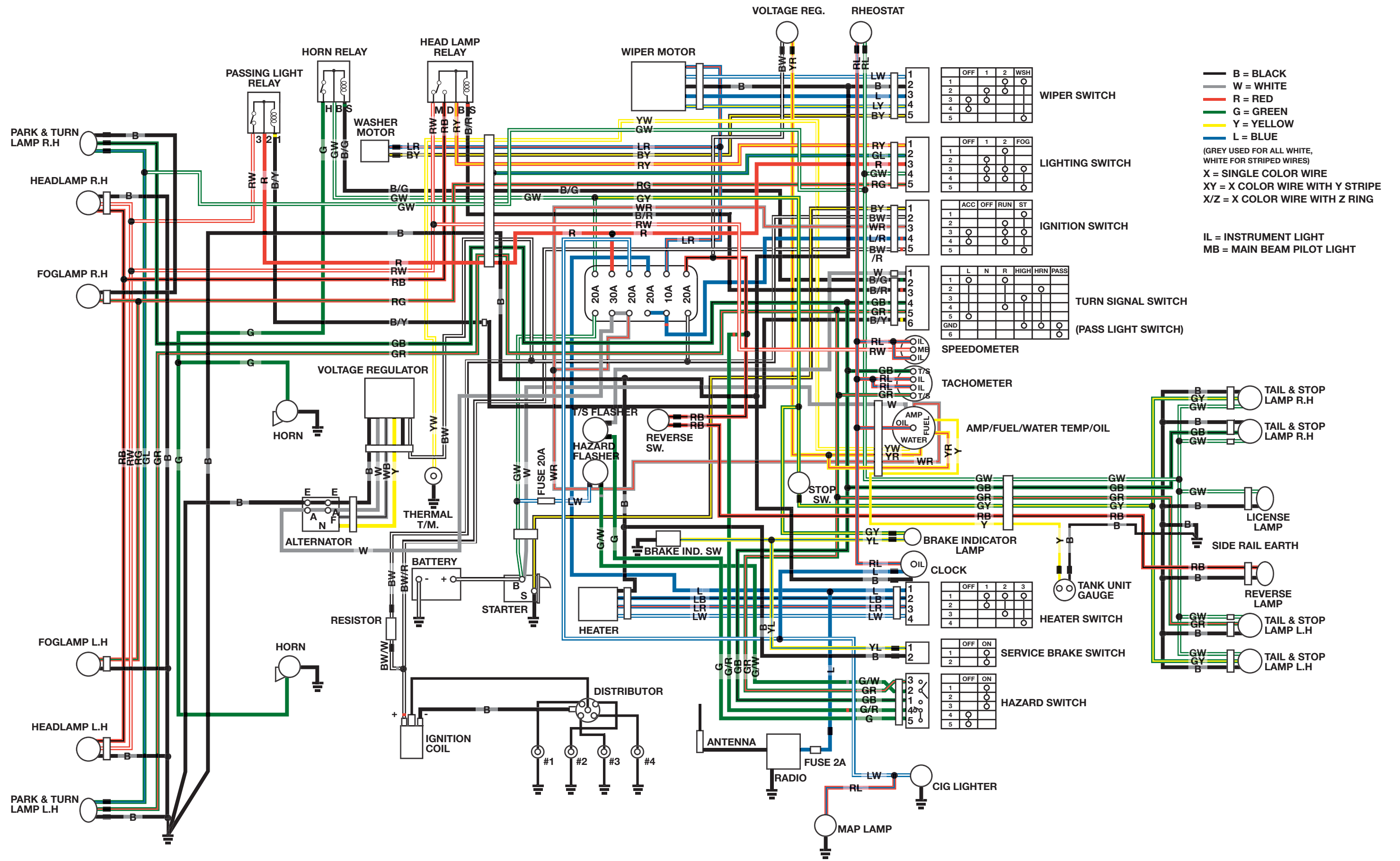
WIRING DIAGRAM DATSUN SPL311 & SRL311 (HIGH WINDOW 1968)
